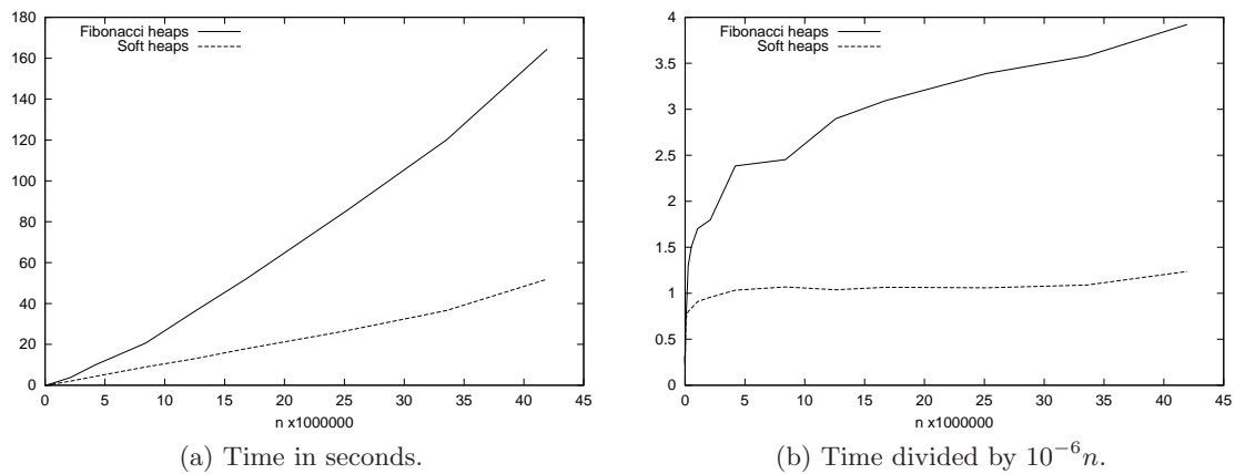
Figure 18.3: Time for mixed heap operations.
