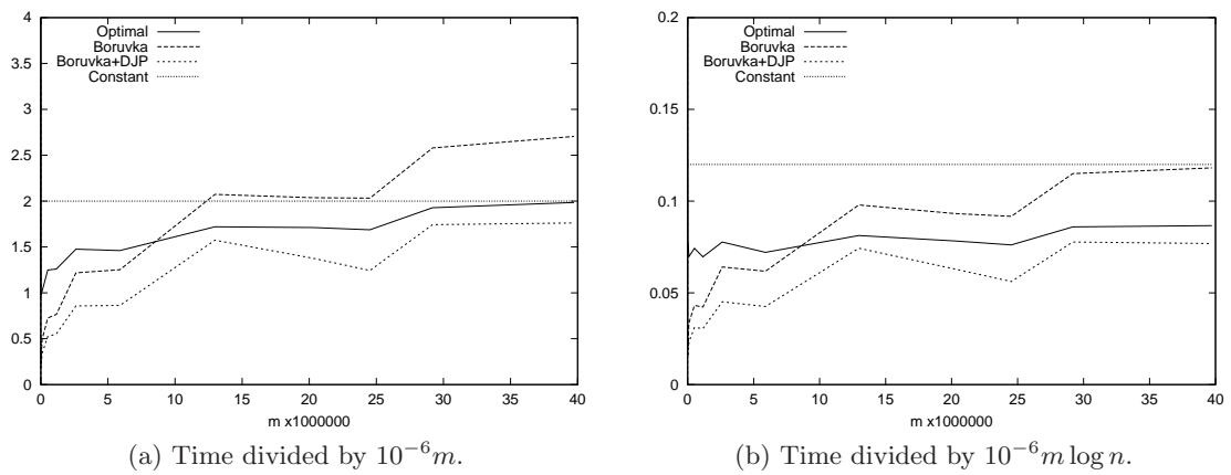
Figure 19.11: Running times for the Borůvka worst case graph.
