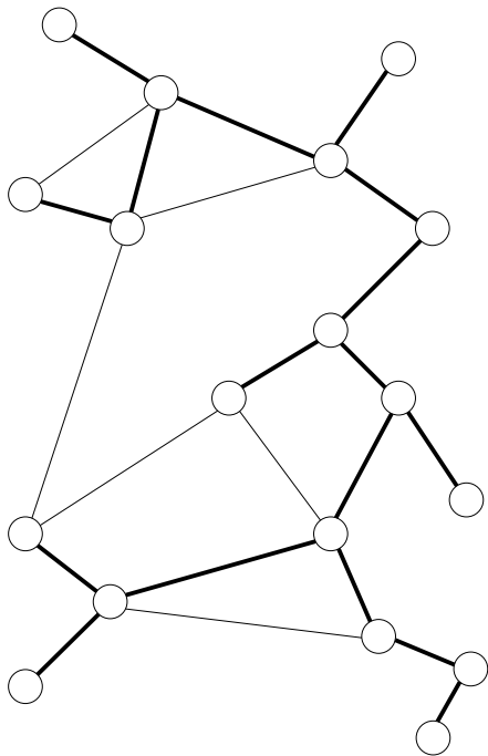
(a) Candidate edges G_b context.
