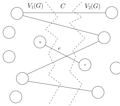
(b) The cut property. Only edges in the cut C are shown.
