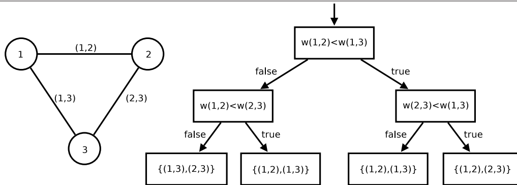
Figure 11.1: A graph with n = 3 vertices defined by ((1, 2), (1, 3), (2, 3)) and its hardwired optimal decision tree.
