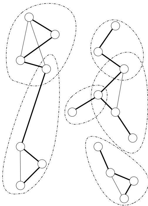
Figure 15.3: After DecisionTree.
