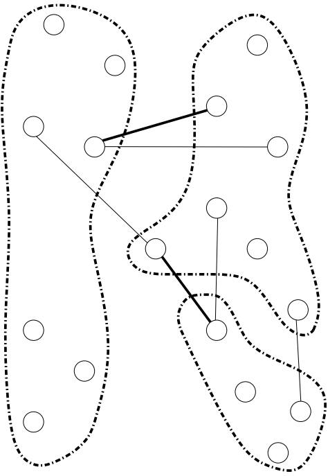
Figure 15.5: After DenseCase.
