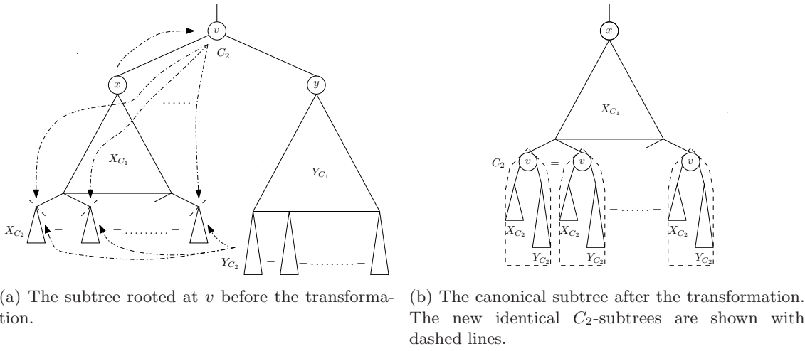
Figure 15.10: The node v has an intra- C_2 comparison associated. In this example, the left subtree X_{C_1} of v has minimum height. So we must copy the comparison of v to each node in a new level of leaf nodes in X_{C_1} , and replace v by x . Additionally we must make X_{C_2} (respectively, Y_{C_2} ) the left (respectively, right) child of each new leaf.
