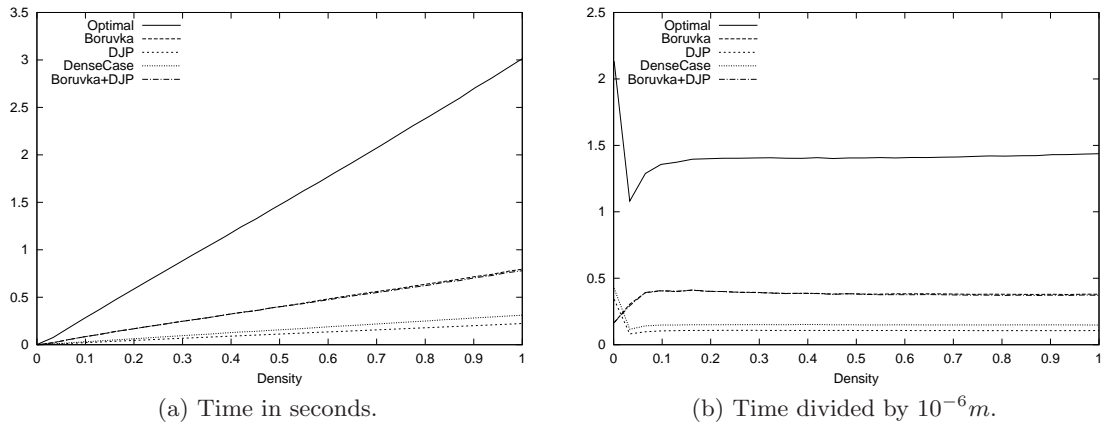
Figure B.6: Constant n = 2^{11} = 2048 .
