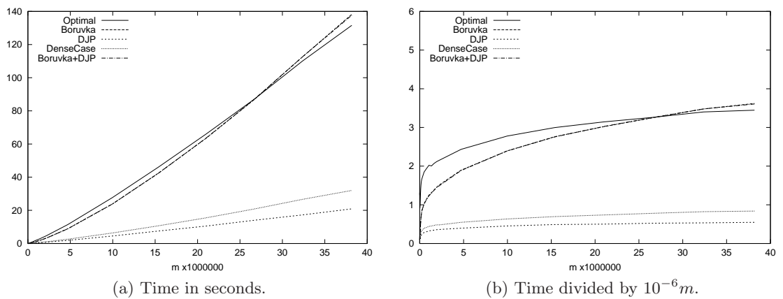
Figure B.2: Constant density, m = n \log n .
