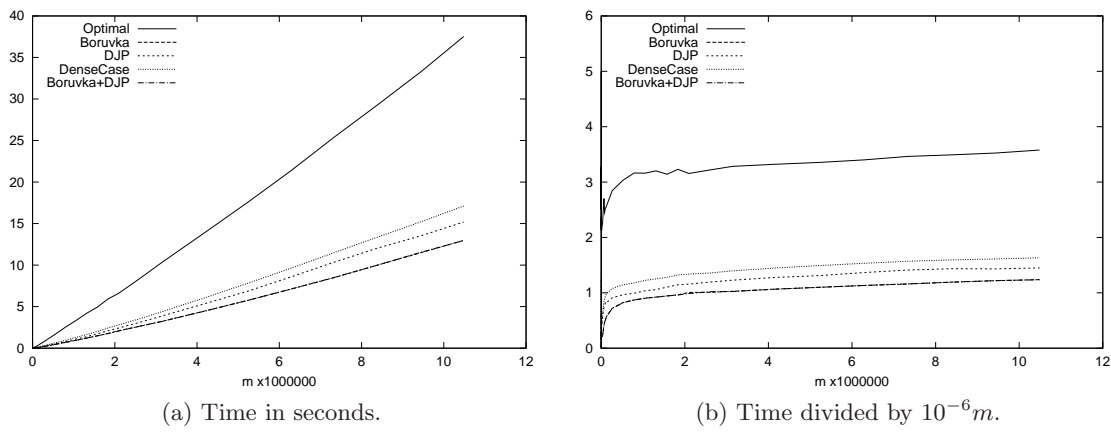
Figure 19.1: Constant density, m = n .
