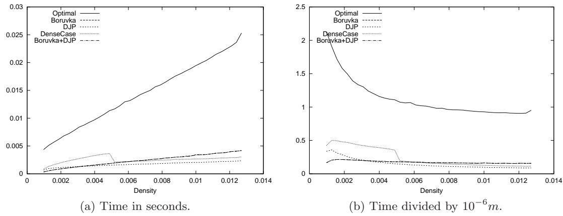
Figure B.9: Constant n = 2^{11} = 2048 , sparse.
