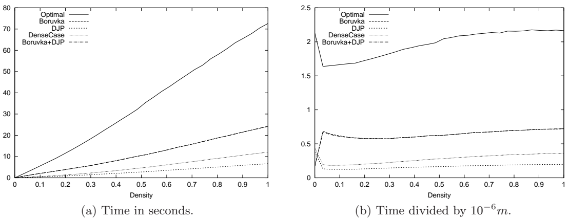
Figure B.7: Constant n = 2^{13} = 8192 .
