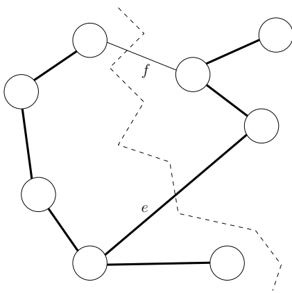
(a) The cycle property. The fat edges are the assumed MST. The dashed line illustrates the splitting of the tree.
