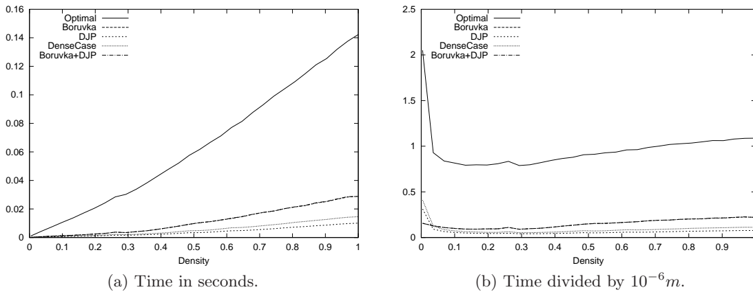
Figure 19.5: Constant n = 2^9 = 512 .
