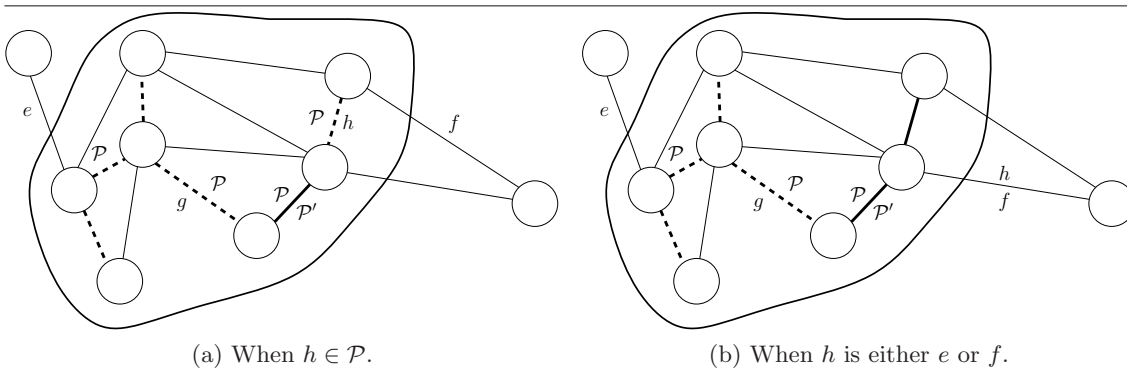
Figure 14.1: Proof of Lemma 14.1. Edges in T are fat. Edges in T' are solid. Edges in (T - T') are dashed.
