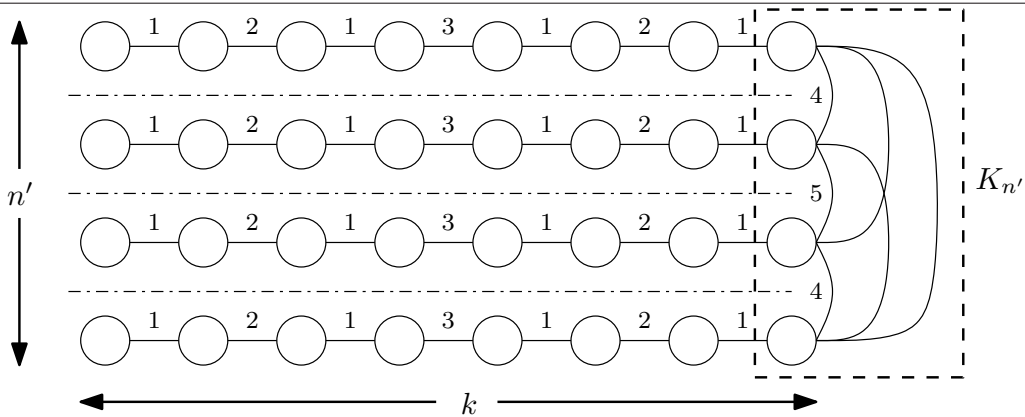
Figure 19.9: Borůvka worst case graph with k = 8 and n' = 4 .
