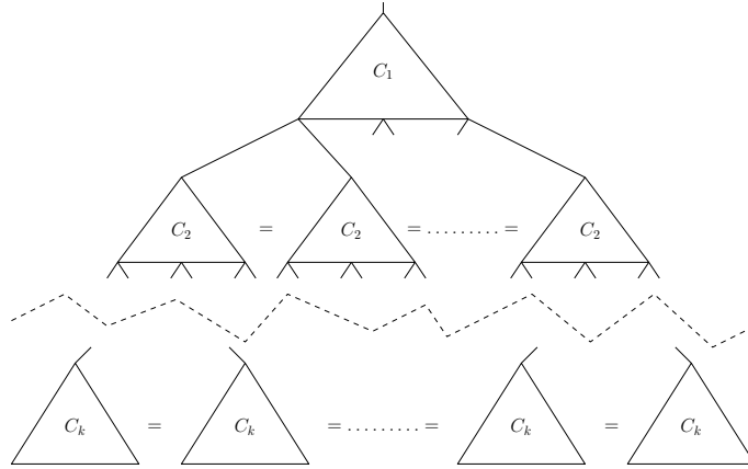
Figure 15.8: Canonical decision tree for H with k components.
