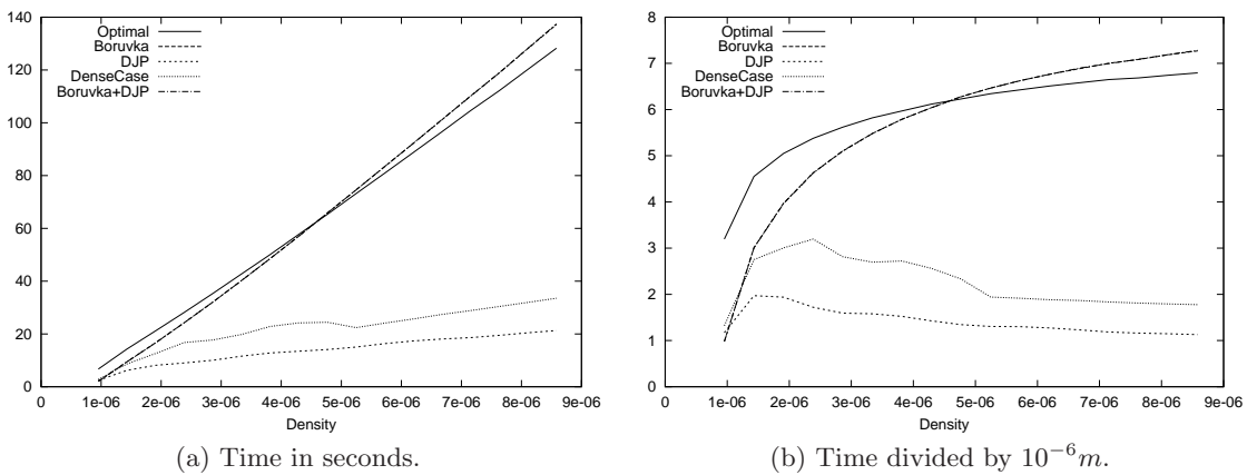
Figure 19.8: Constant n = 2^{21} , sparse.
