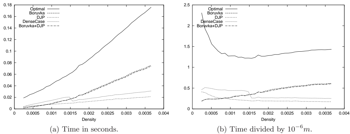
Figure B.10: Constant n = 2^{13} = 8192 , sparse.
