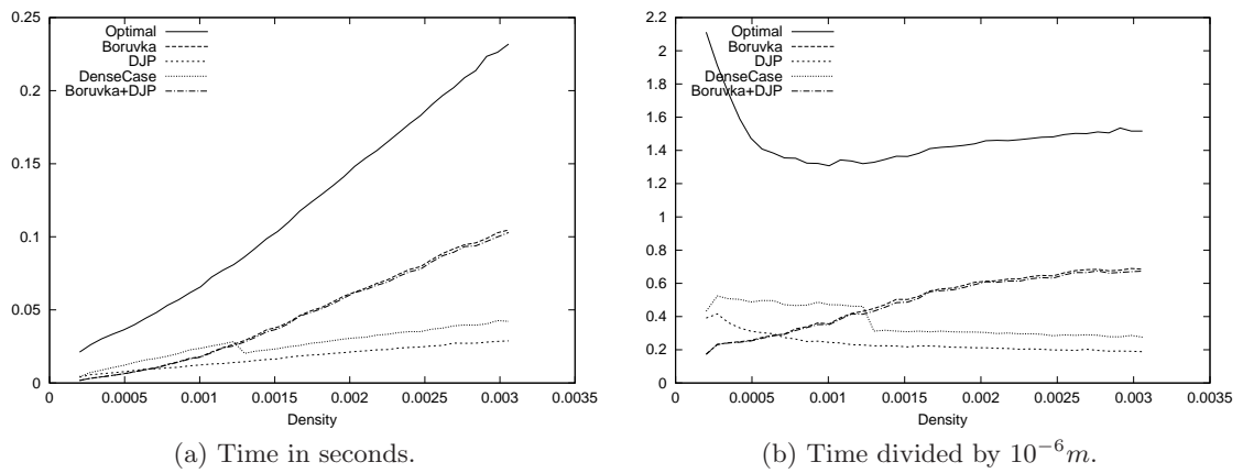
Figure 19.7: Constant n = 10^4 = 10000 , sparse.
