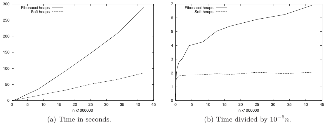
Figure 18.2: Time for heap deleteMins
