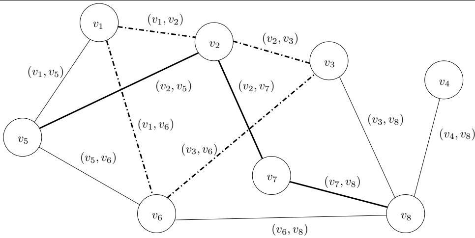
Figure 3.1: A simple connected graph G with n = 8 and m = 12 , defined by V = \{v_1, \dots, v_8\} and E = \{(v_1, v_2), (v_1, v_5), \dots, (v_6, v_8), (v_7, v_8)\} . A sequence as (v_5, (v_2, v_5), v_2, (v_2, v_7), v_7, (v_7, v_8), v_8) (bold edges) forms a simple path. A sequence as (v_2, (v_2, v_3), v_3, (v_3, v_6), v_6, (v_1, v_6), v_1, (v_1, v_2), v_2) (dash-dotted edges) forms a simple cycle.
