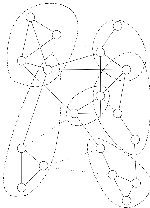
Figure 15.2: After Partition.
