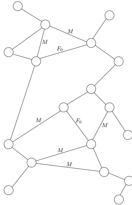
Figure 15.6: Candidate edges G_b .
