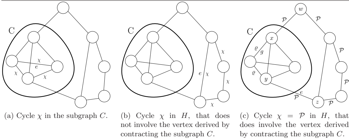
Figure 14.2: Proof of Lemma 14.2.
