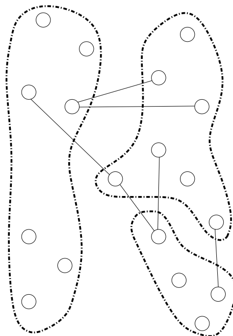
Figure 15.4: The contracted graph G_a .
