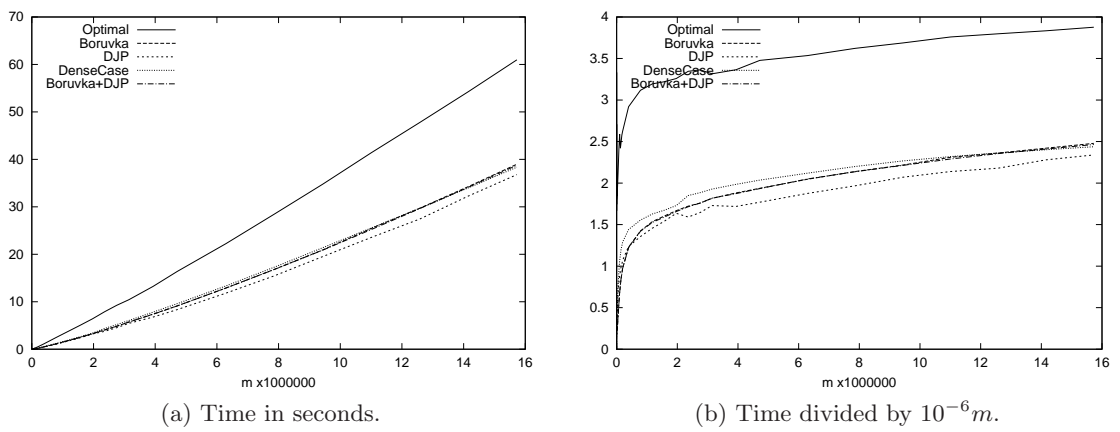
Figure B.1: Constant density, m = 1.5n .
