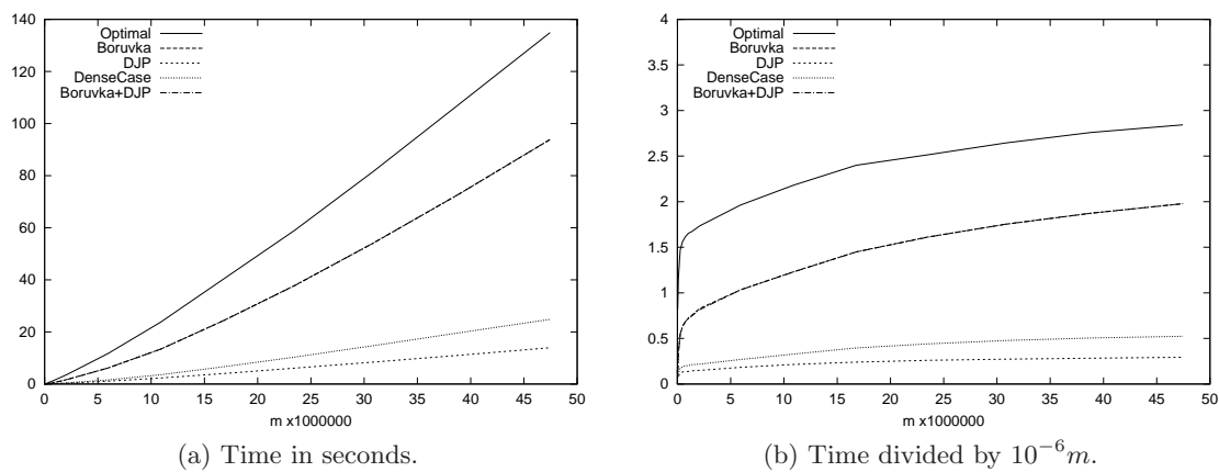
Figure 19.3: Constant density, m = n\sqrt{n} .
