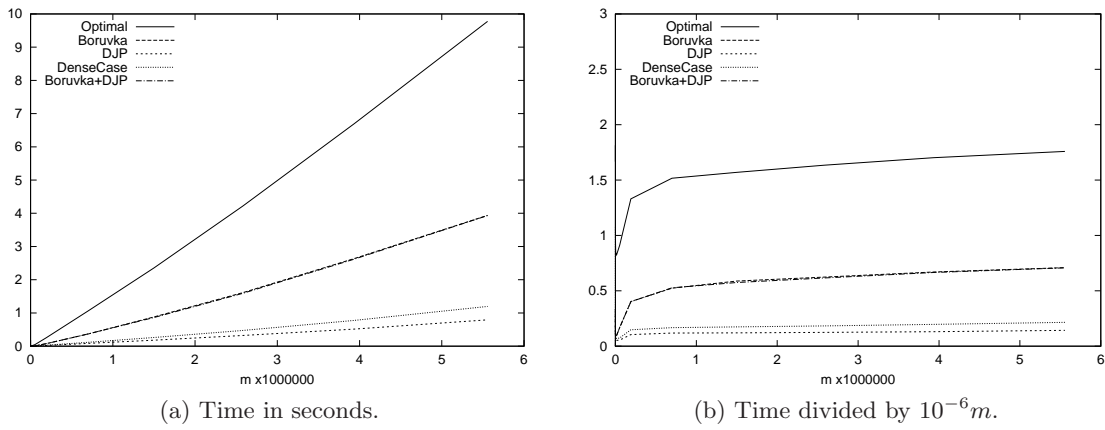
Figure B.3: Constant density, m = m_{\max}/\log n .
