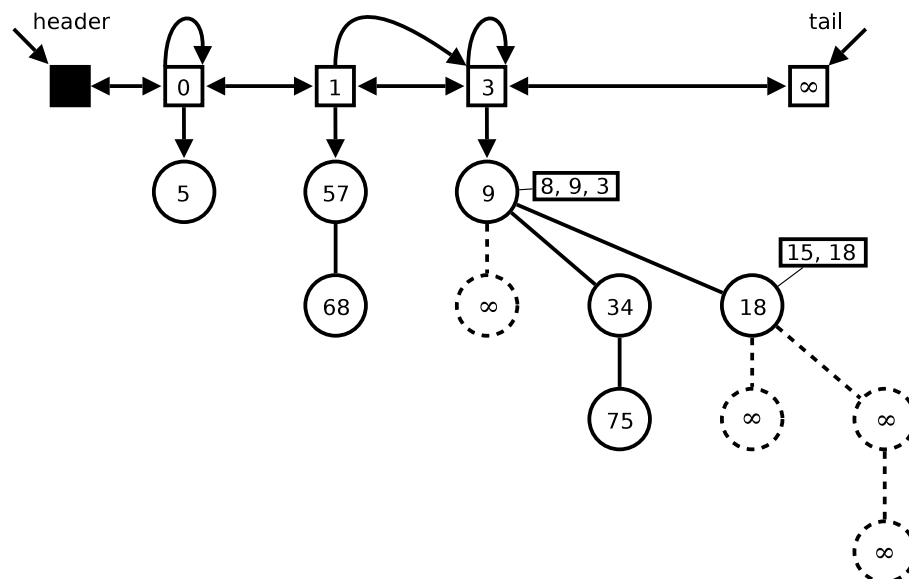
Figure 12.1: Soft heap data structure with three soft queues. The number inside a squared head is the queue rank. The number inside a queue node is the ckey . The item lists with size > 1 is shown next the queue node. Removed subtrees are shown with dashed lines.
