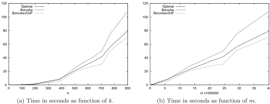
Figure 19.10: Running times for the Borůvka worst case graph.
