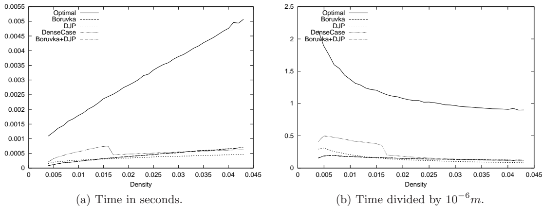
Figure 19.6: Constant n = 2^9 = 512 , sparse.
