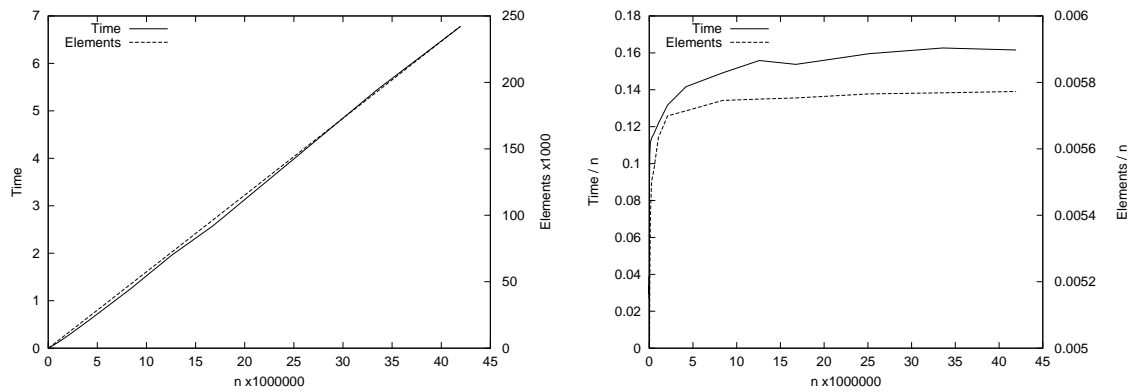
(a) Time in seconds and the number of corrupted elements. (b) Time divided by 10^{-6}n and number of corrupted elements divided by n .
