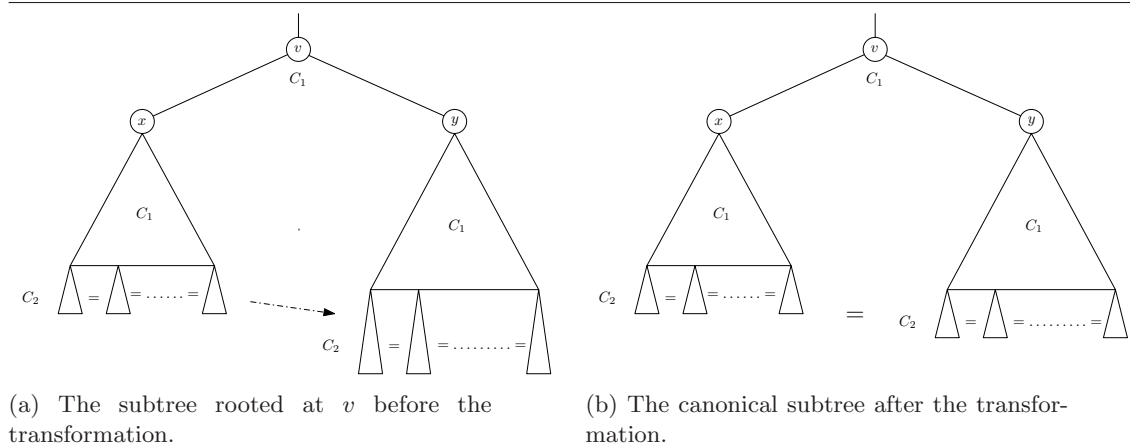
Figure 15.9: The node v has an intra- C_1 comparison associated. In this example, the C_2 -subtrees under x has minimum height. Hence, all C_2 subtrees must be replaced by such subtree.
