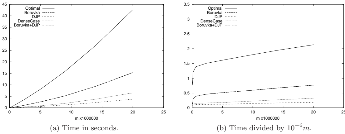
Figure B.4: Constant density, m = m_{\max}/\log \log n .
