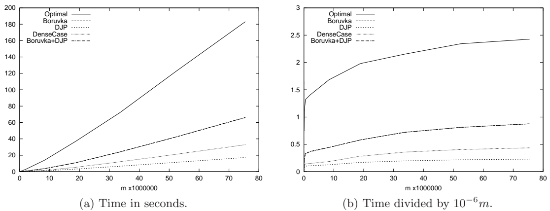
Figure 19.4: Constant density, m = m_{\max} .
