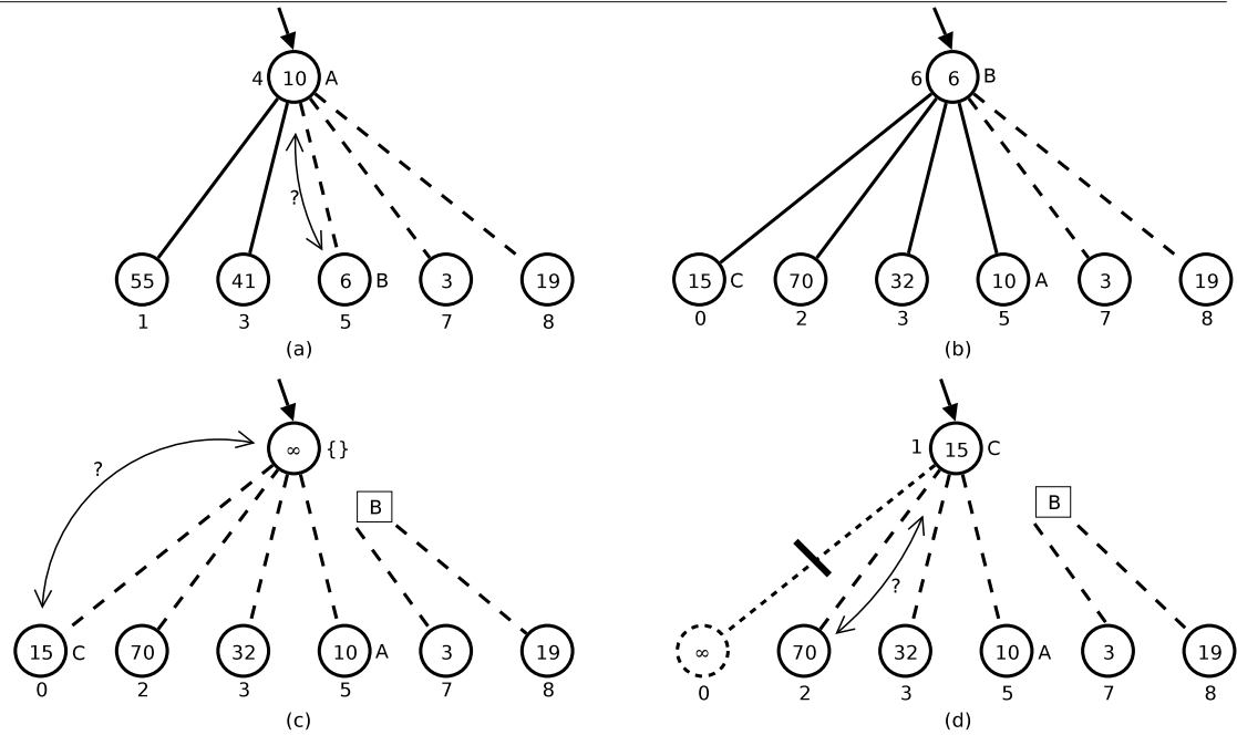
Figure 12.2: Example of sifting, starting in a relinking iteration. Only the current root and subtree roots are shown. Unlinked subtrees are shown with dashed lines to the root. The number inside a node is the ckey . The number below a subtree root is the rank. The number next to the root is the current root rank. The letter next to some nodes is the item list. a) 10 is just linked with 41. 10 and 6 is about to be linked. b) 10 and 6 linked. The root has lost the child of current rank 6, so we call recursive. c) Recursive call: The current unlinked subtrees (3 and 19) are unknown to the recursive call. The item list ( B ) at the root is saved, illustrated by the new box. Then the item list at the root is emptied, the ckey is set to \infty , and the current children are unlinked. The root and 15 is about to be linked. d) 15 and \infty not linked, but \infty is removed. The next linking step will involve 15 and 70. Assuming no further recursive calls occur, this recursive call will end by swapping the root (15) and 10, making 10 the new root, and merging the items lists A and B .
