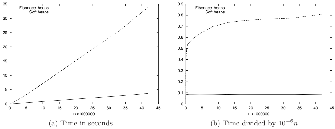
Figure 18.1: Time for heap insertions.
