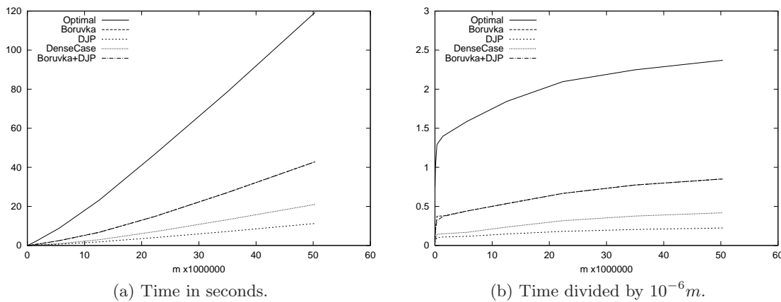
Figure B.5: Constant density, m = m_{\max}/1.5 .
