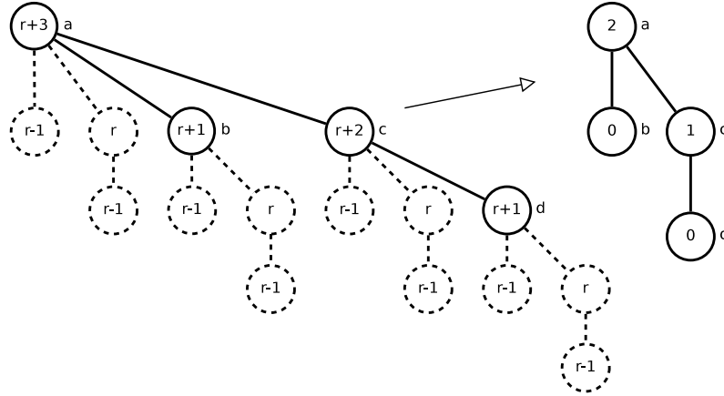
Figure 12.3: To the left: A binomial tree, q' , with node ranks. The nodes in R'_{q'} have solid lines. To the right: The binomial tree formed by nodes in S_{q'} with node ranks.
