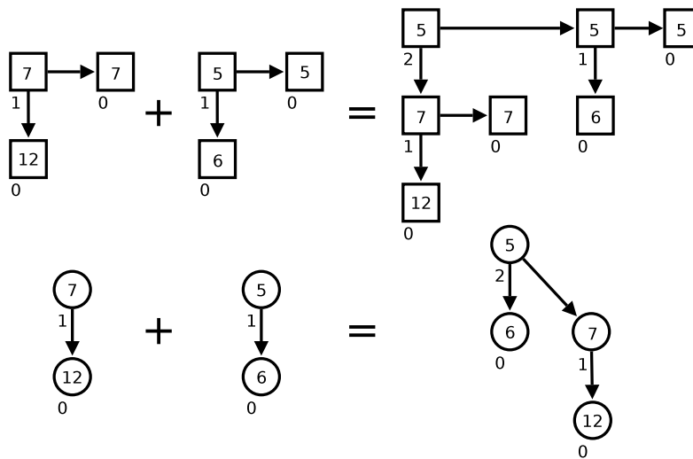
Figure 12.4: Linking of two binomial queues with rank 1. The number inside a node is the ckey . The number below a node is the rank. Top: Chazelle's representation. Bottom: Standard view.
