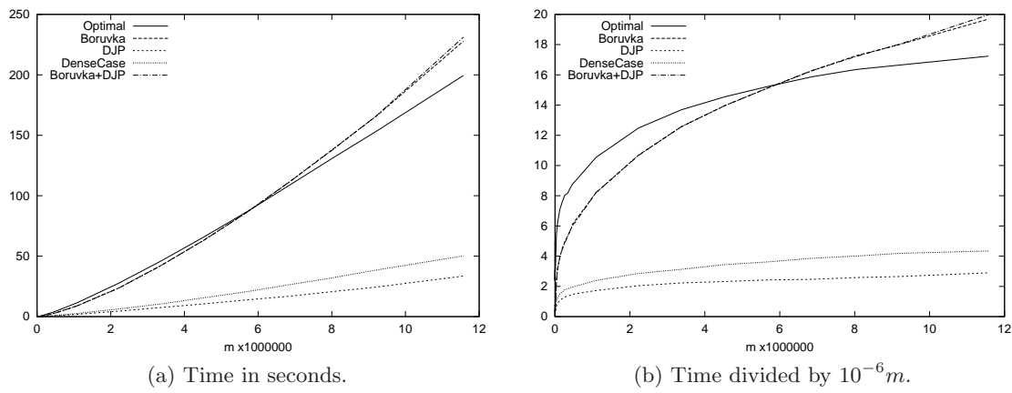
Figure 19.2: Constant density, m = n \log \log n .
